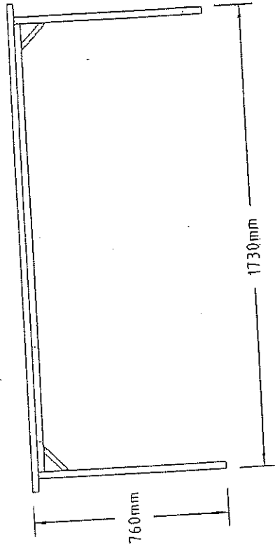
PANDANGAN HADAPAN
