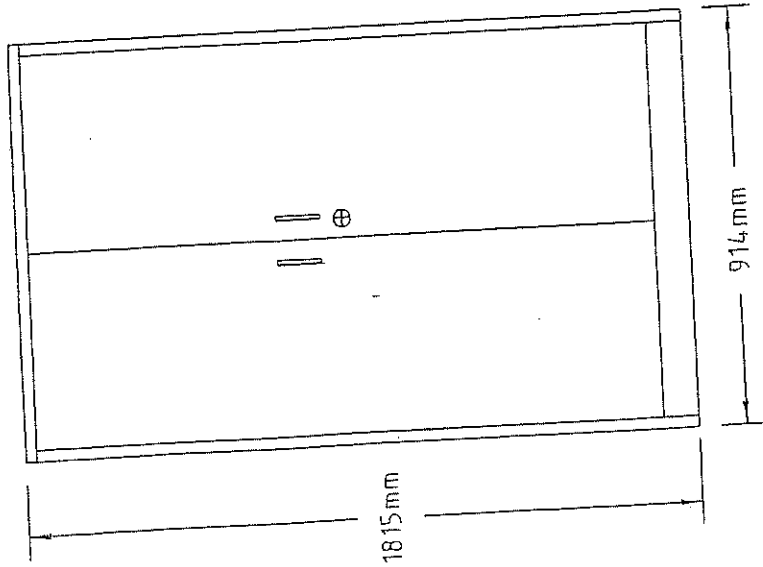
PANDANGAN HADAPAN
