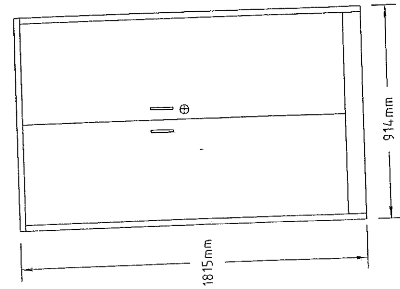
PANDANGAN HADAPAN
