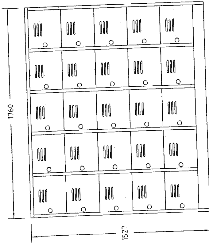
PANDANGAN HADAPAN
